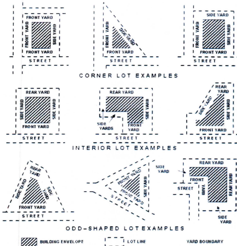
Figure 1 Examples for identifying front, rear, and side yards
